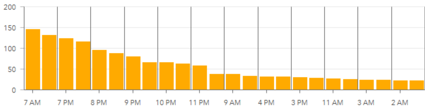
Time of Day
