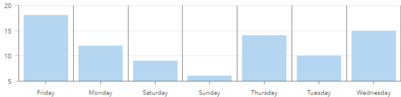
Dear Crashes per Day of the Week
