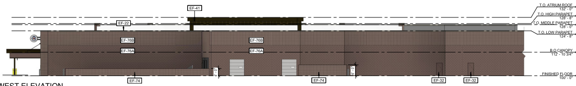
C1 WEST ELEVATION SCALE: 1/16" = 1'-0"
