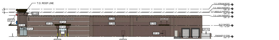
B1 NORTH ELEVATION SCALE: 1/16" = 1'-0"
