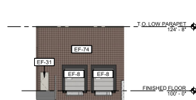
A1 TRUCK DOCK ELEVATION SCALE: 1/16" = 1'-0"
