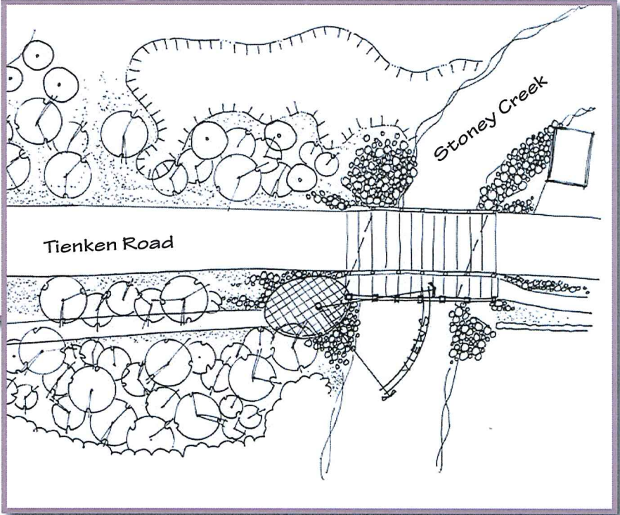
Concept of the non-motorized path attached to the south side of the Stoney Creek Bridge. ▶
