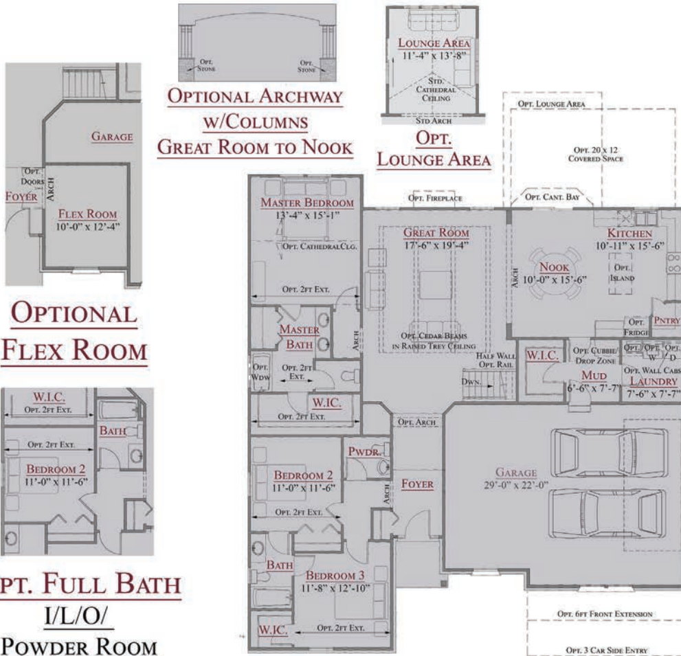
FLOOR PLAN
