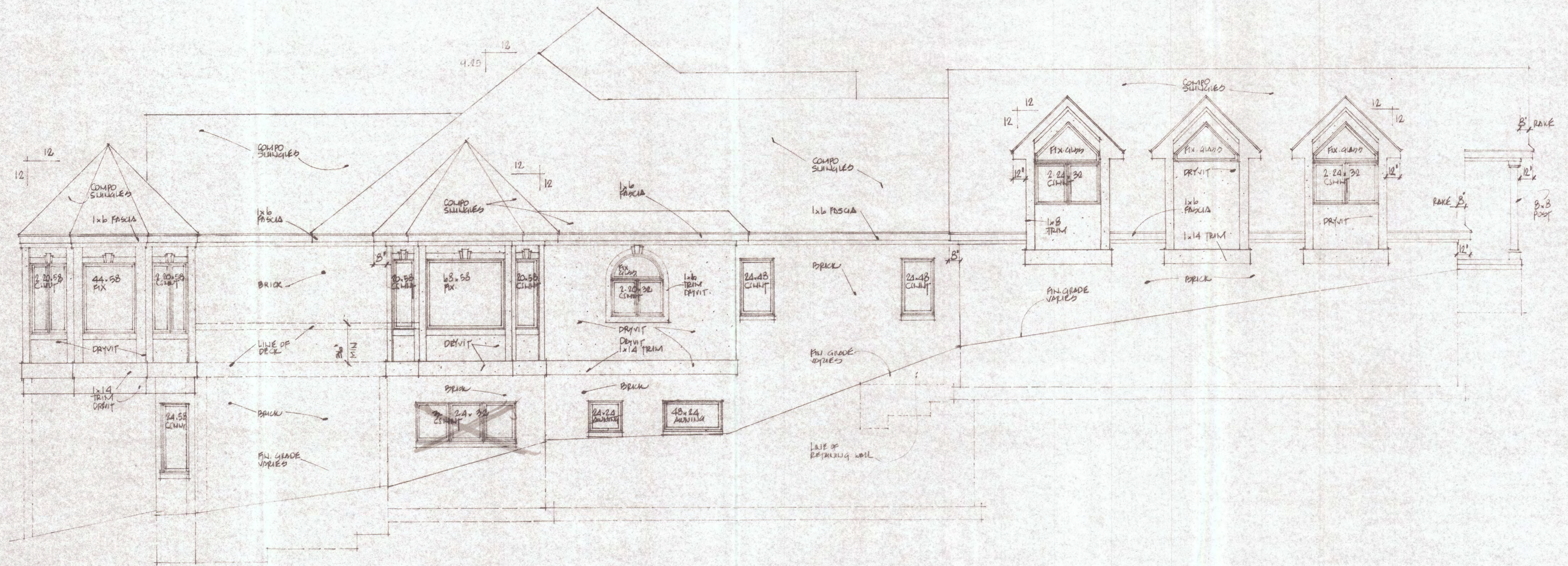
LEFT SIDE ELEVATION SCALE: 1/4" = 1'-0"
