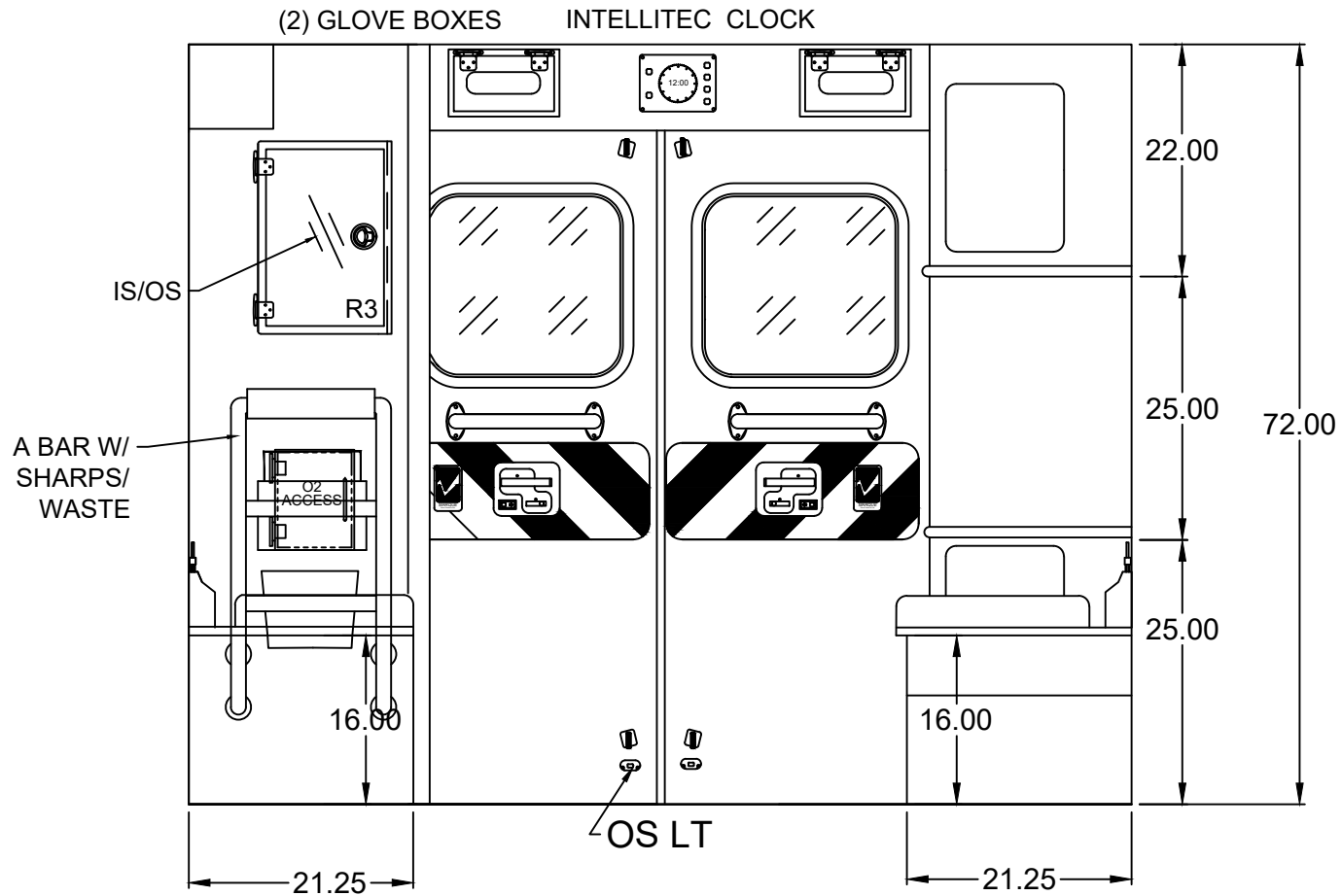
CABINET SIZES INSIDE DIMENSIONS
