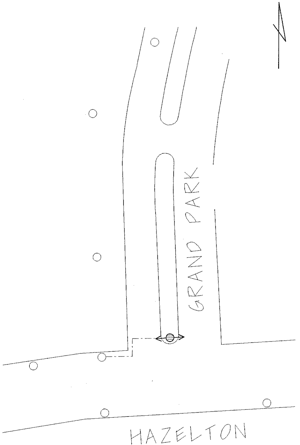
12-FOOT FIBERGLASS "WINDSOR" POST WITH TWIN 100-WATT HPS ACORN LUMINAIRES
