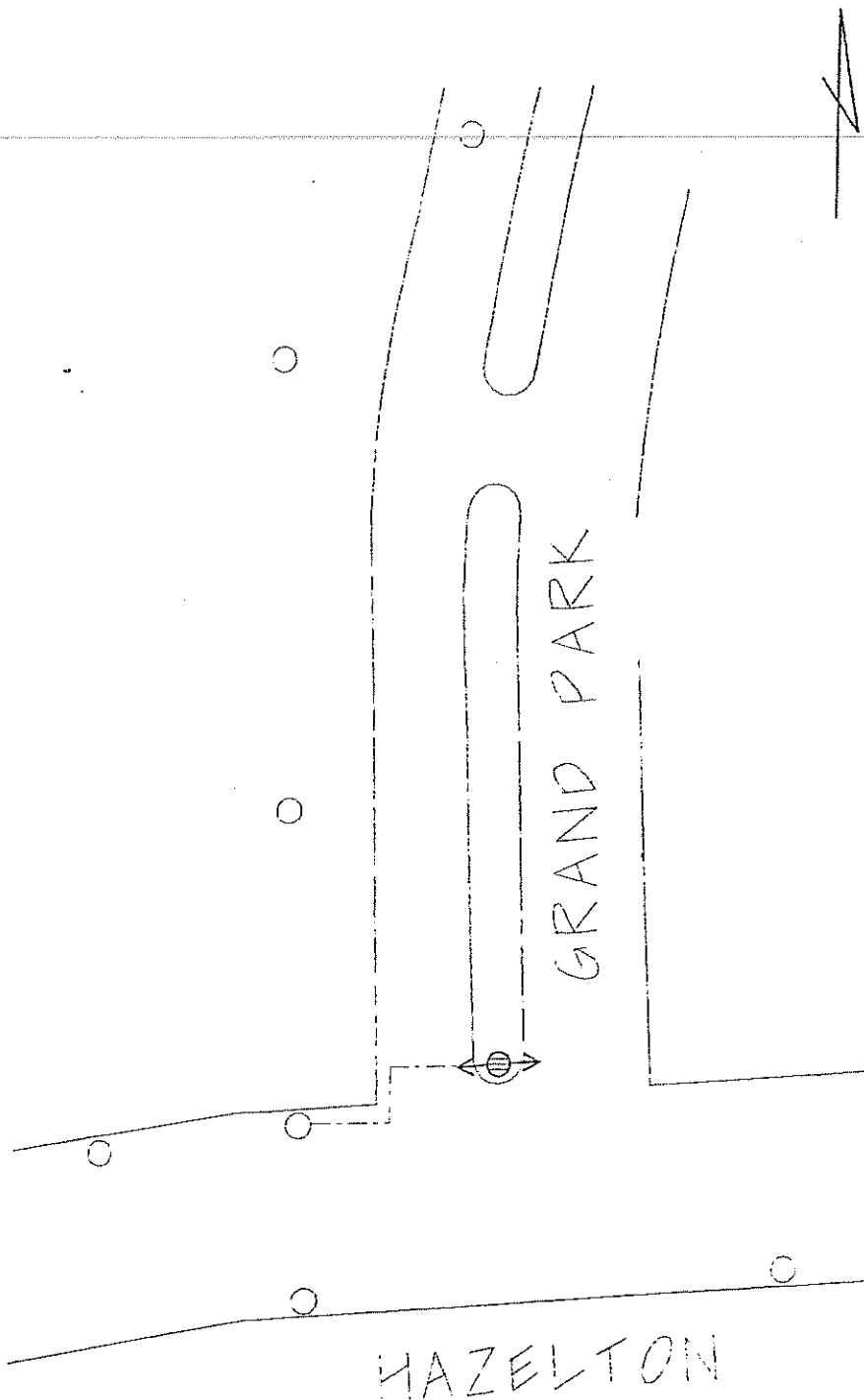
12-FOOT FIBERGLASS "WINDSOR" POST WITH TWIN 100-WATT HPS ACORN LUMINAIRES
