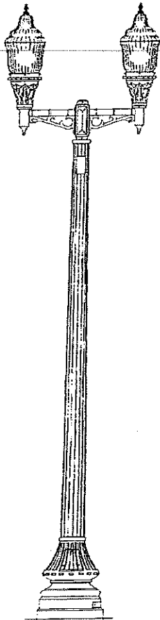
12-FOOT FIBERGLASS "WINDSOR" POST WITH TWIN 100-WATT HPS ACORN LUMINAIRES
