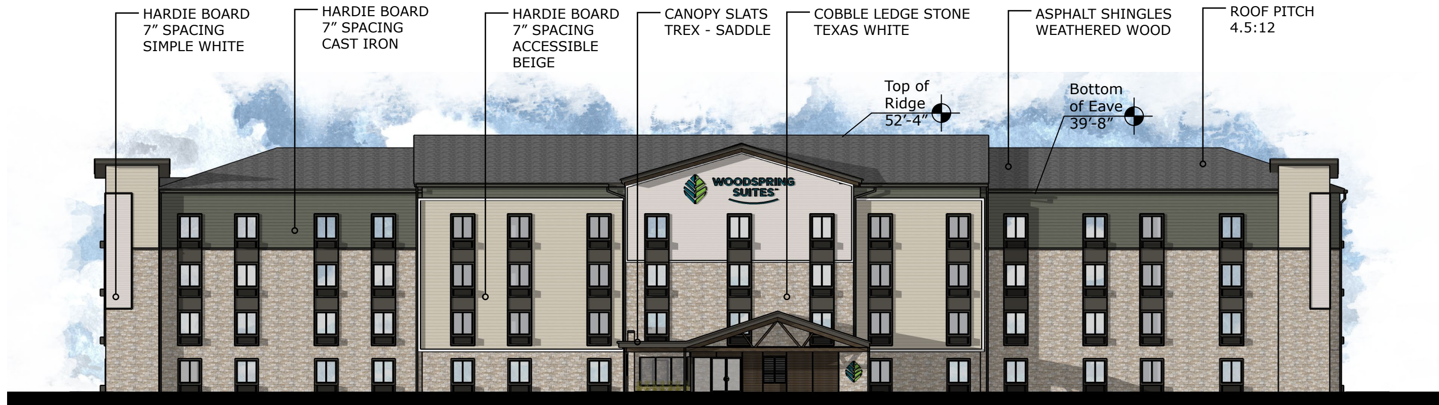
Front Elevation
