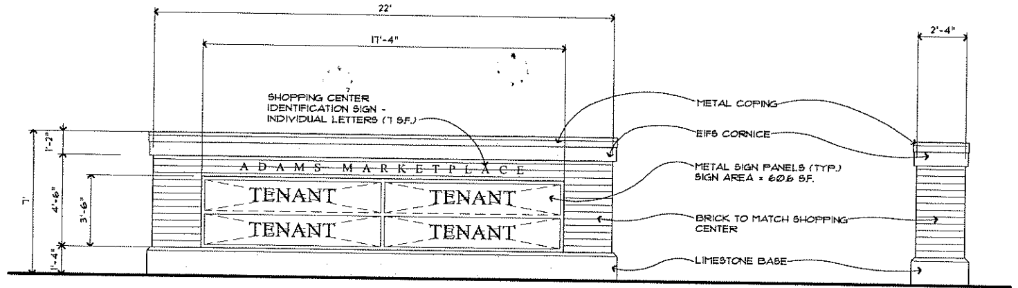
FRONT ELEVATION
