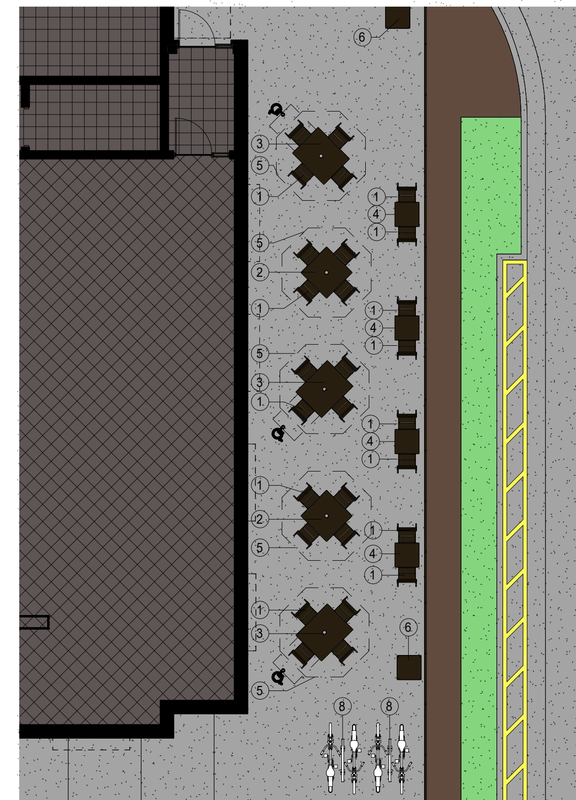
DINING PATIO PLAN 1/8" = 1'-0"
